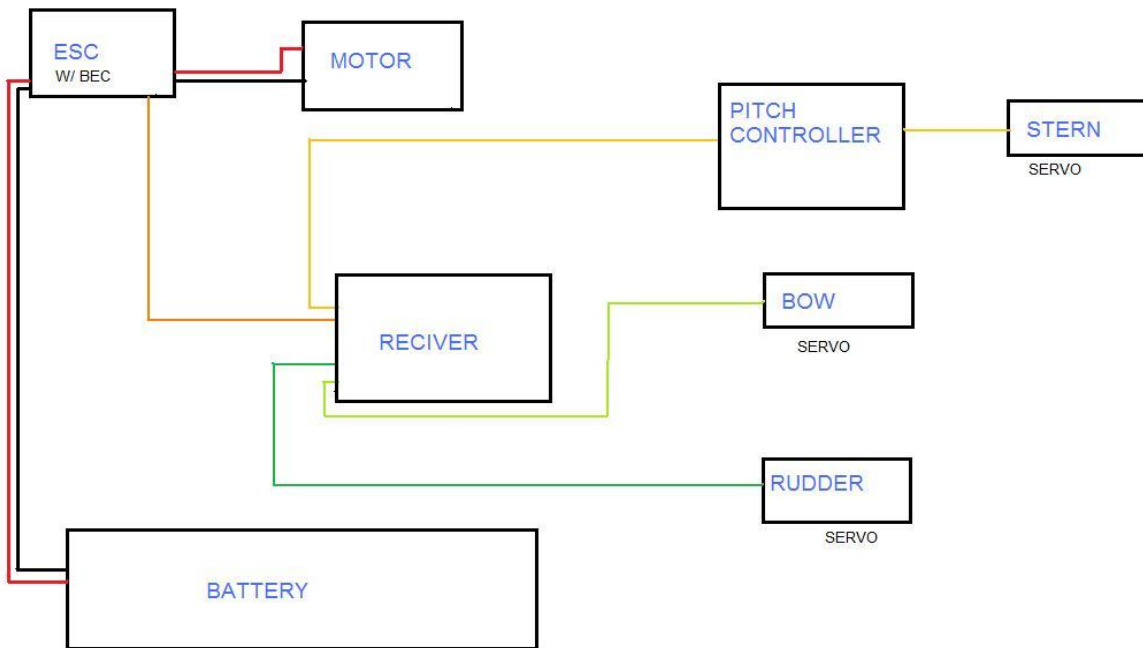
BASIC DYNAMIC DIVING SUBMARINE DIAGRAM
